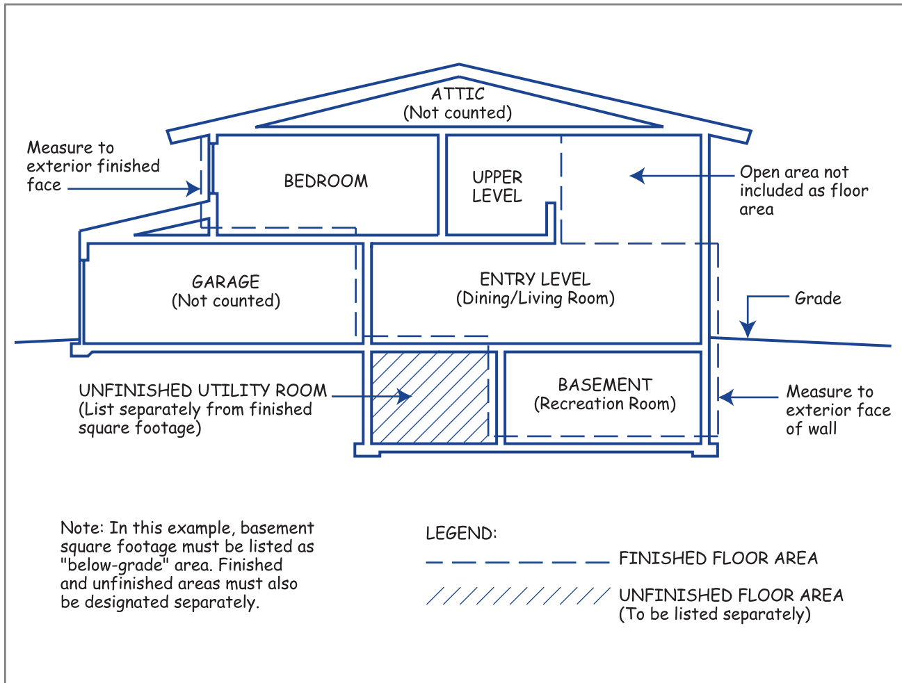
FIGURE 4. Building Section
